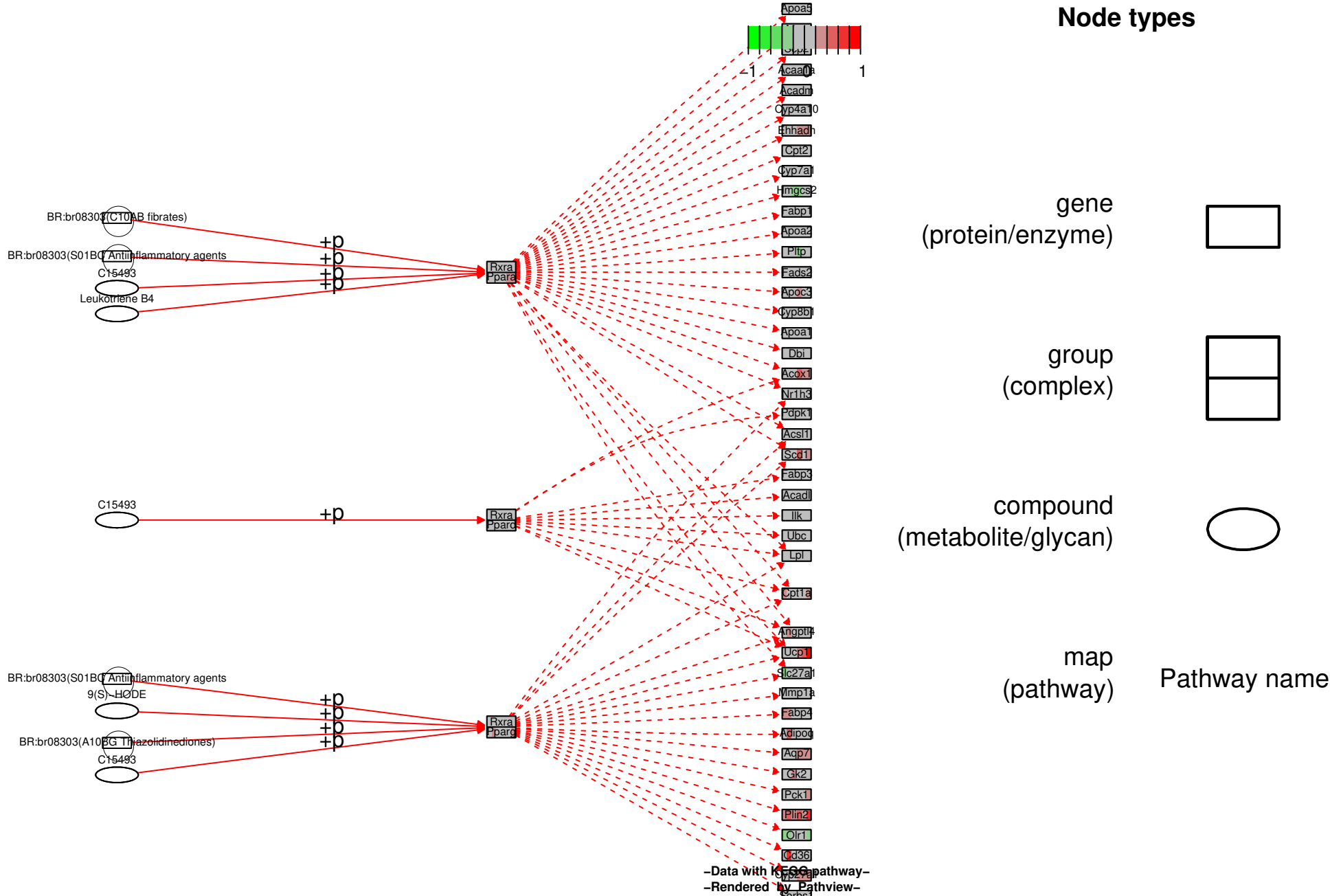
Graphviz representation of PPAR signaling pathway (mmu03320). Box of expressed genes are colored according to the scaled log 2 FC between epi and ing expression levels. Each box is partitioned into six parts, each representing one time point (-2,0,2,4,6,8), so that the whole time course for the gene is shown. The log 2 FC is scaled between -1 to 1. When the gene is higher expressed in ing the color is in a shade of green, while it is red, when the gene is higher expressed in epi. Grey color indicates a similar expression intensity in both adipose tissues, and no filling means no expression was measured.
